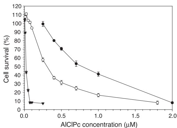
Fig. 3. Survival of EMT-6 cells upon PDT treatment after 1 h of incubation with AICIPc loaded micelles. Randomly alkylated copolymer ( \blacktriangledown ); terminally alkylated copolymer (O); Cremophor EL ( \bullet ). (Reproduced with permission from [33].)
