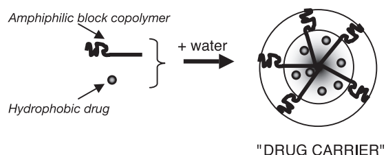
Fig. 1. Schematic representation of the micelle formation and drug-loading of amphiphilic block copolymers in water.
