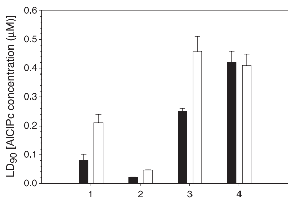
Fig. 4. Dose of AICIPc in micelles required to inactivate 90% of EMT-6 cells ( LD_{90} ) upon PDT treatment after 24 h of incubation with (white bars) or without (black bars) 50 \mu\text{M} chloroquine. Randomly alkylated (2 mol%) copolymer containing 5 mol% (1) and 3 mol% MAA (2); terminally alkylated copolymer (3); Cremophor EL (4). (Reproduced with permission from [33].)
