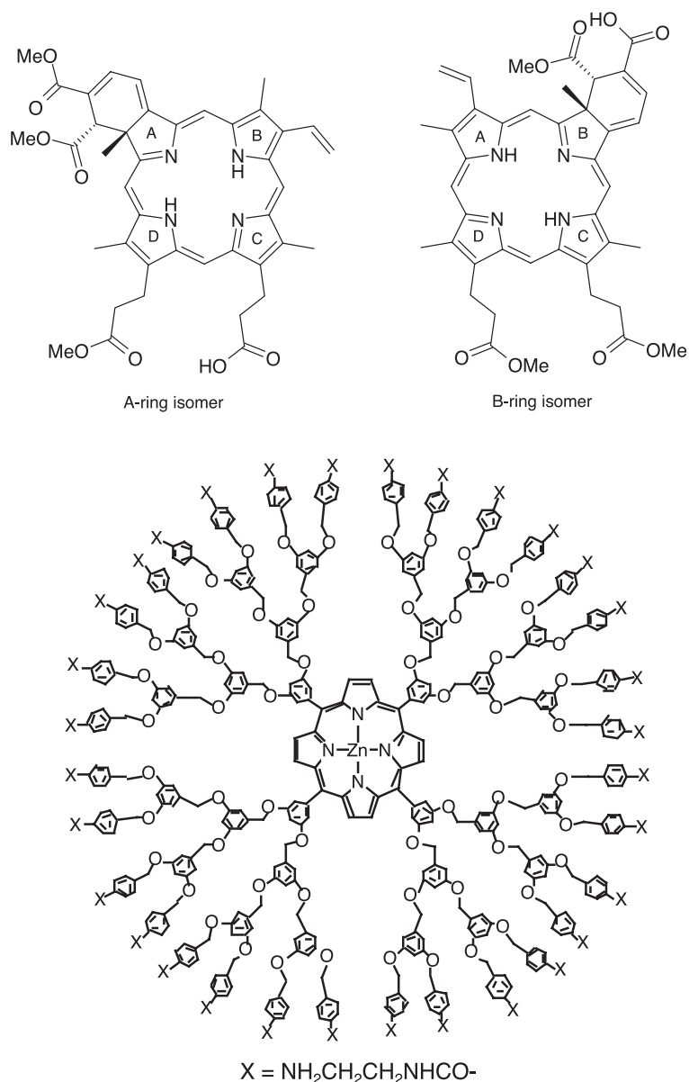
Fig. 2. Structural formulas of A- and B-ring isomers of benzoporphyrin (top) and zinc porphyrin dendrimer (bottom).
